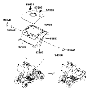
F08 Body Cover
